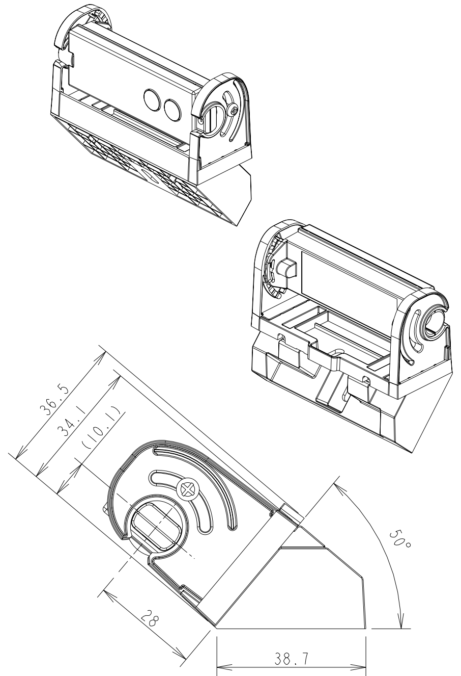
KT-RC2 Sensor Unit with spacer outline drawing 2016.05.13 NEC Display Solutions, Ltd.
